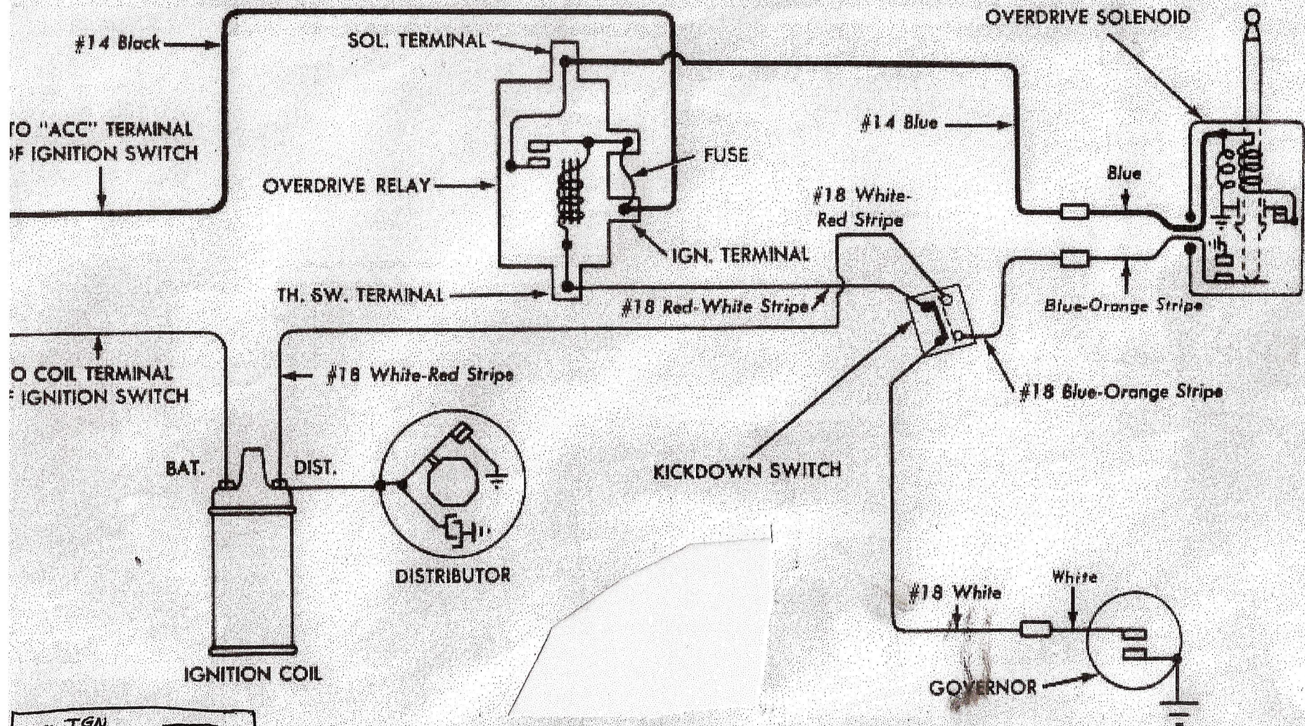
Overdrive electrical system (© Borg Warner Corp.)
